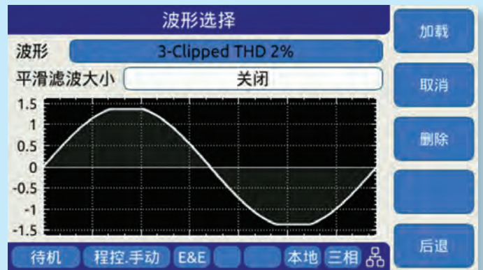
交流输出波形选择 - Vthd = 10%
